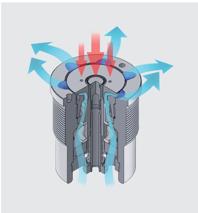
Nozzle function in case of blocked rotor
